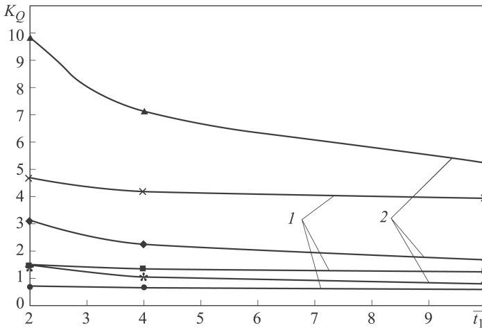
Fig. 9. Dependency of the efficiency criterion K_Q on the finning pitch at various angles and Biot numbers ( Re = 10^4 ; \bar{h}_1 = 4 ): curves 1 ( Bi=0.4 ) – \bullet – \beta = 20^\circ ; \blacksquare – \beta = 30^\circ ; \times – \beta = 45^\circ ; curves 2 ( Bi=0.04 ) – * – \beta = 20^\circ ; \blacklozenge – \beta = 30^\circ ; \blacktriangle – \beta = 45^\circ
