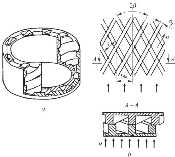
Fig. 1. Coplanar channel:
